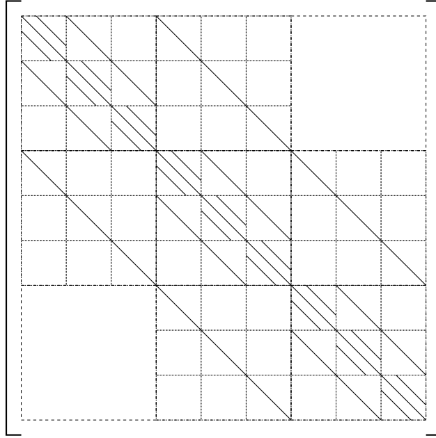
Figure 1: Banded matrix produced by the box-method.
